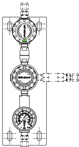
Special C with check valve
