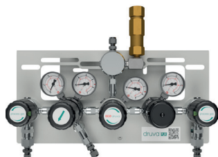
Type MPLH0SDS0U S0 HP Shut-off Valve U Specials Check Valve & Safety Valve
