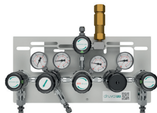
Type MPLH0SDSSU SS HP Shut-off Valve & LP Shut-off Valve U Specials Check Valve & Safety Valve
